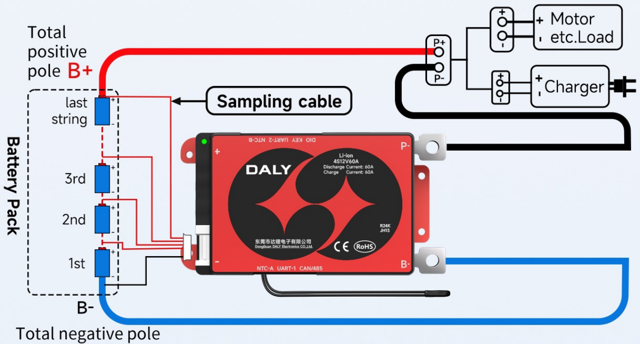
(Wiring Diagram) ⤴
